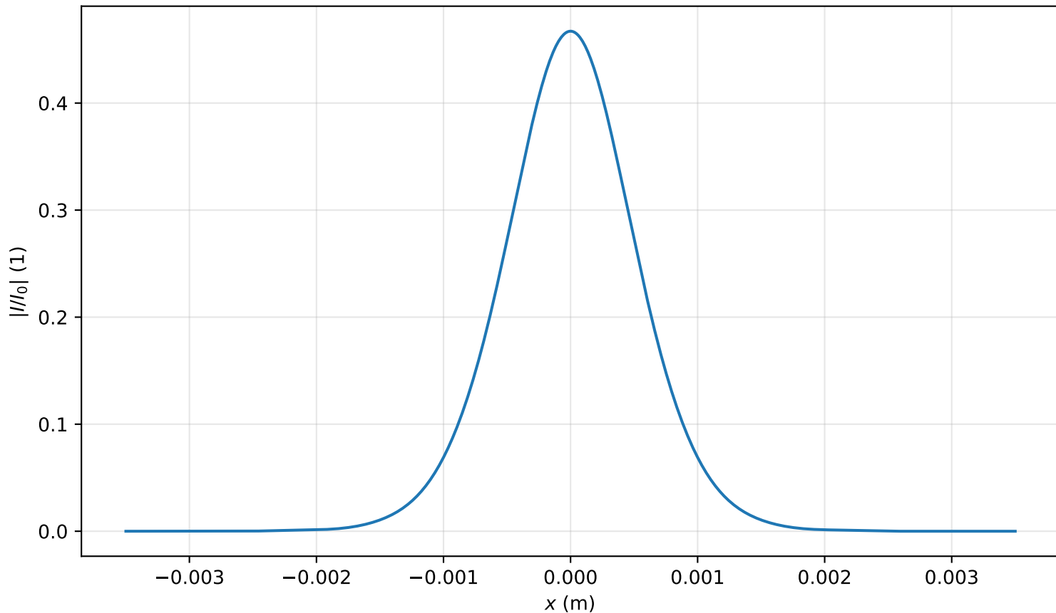
Intensity profile I(x, y = 0, z = 3.503m)/I_0 , P_{in}=0.5P_{cr} , artificial time
